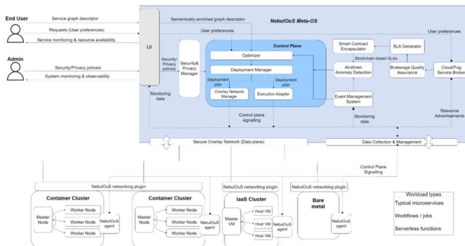
Figure 1: NebulOuS architecture
