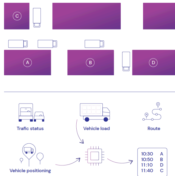
Figure 4: Last mile delivery optimization use case diagram
