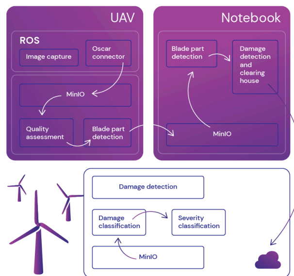
Figure 6: Windmill maintenance use case diagram
