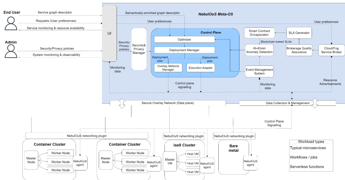
Figure 1: NebulOuS architecture
