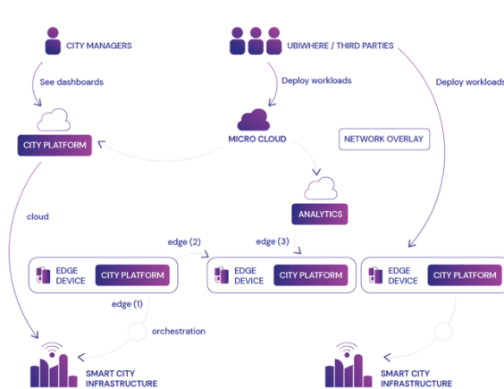
Figure 5: Computer vision for city maintenance use case diagram
